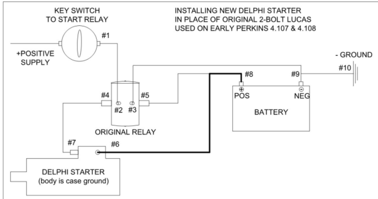
Figure 3 Diagram for connecting Delphi Starter in Place of Lucas Starter
